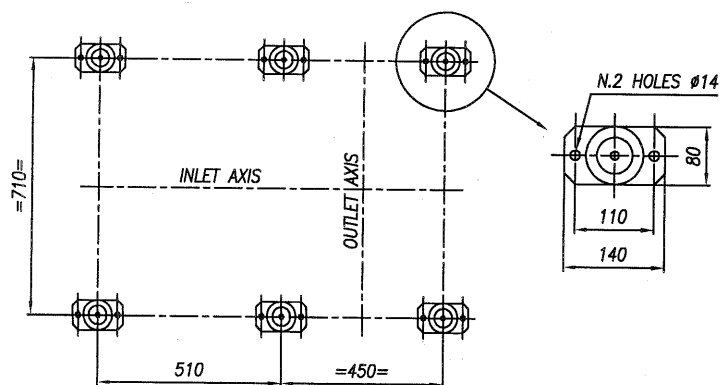
RUBBER ISOLATOR DISPOSITION -TOP VIEW-
