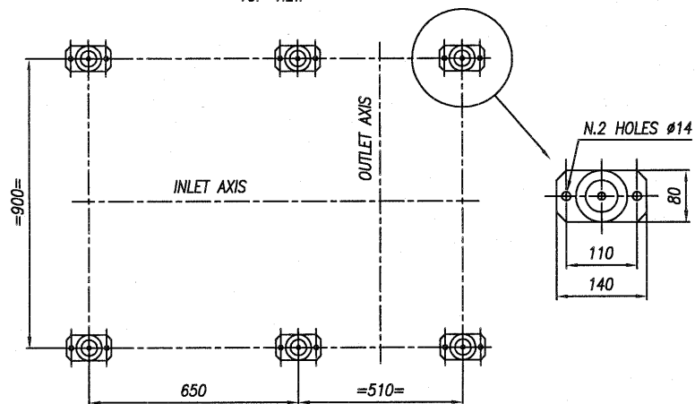
RUBBER ISOLATORS DISPOSITION -TOP VIEW-
