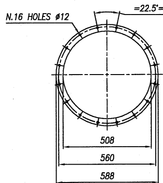
INLET FLANGE
